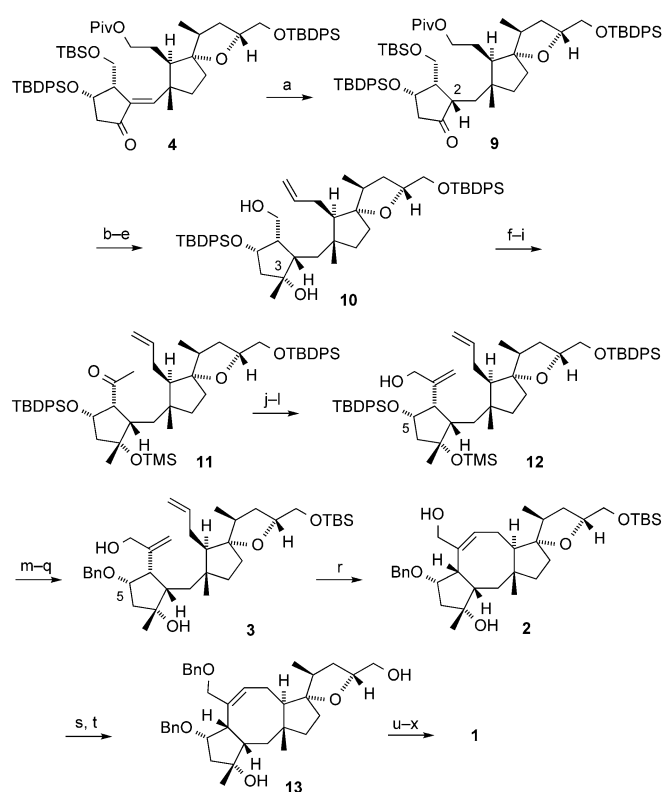
Scheme 3. Total synthesis of (+)-ophiobolin A ( 1 ). a) \text{H}_2 , Raney Ni, MeOH/THF = 1:1, RT, 82%, d.r. = 41:1; b) MeLi, \text{Et}_2\text{O} , -78 to 0^\circ\text{C} , 98%, d.r. = 1:0; c) (\text{COCl})_2 , DMSO, \text{CH}_2\text{Cl}_2 , -78^\circ\text{C} ; then \text{Et}_3\text{N} , RT, 98%; d) \text{Ph}_3\text{P}^+\text{MeBr}^- , t\text{BuOK} , THF, 0^\circ\text{C} , 99%; e) PPTS, EtOH, RT, quant.; f) IBX, DMSO, RT; g) MeLi, \text{Et}_2\text{O} , 0^\circ\text{C} ; h) Dess–Martin periodinane, \text{CH}_2\text{Cl}_2 , RT, 78% (over 3 steps); i) TMSCl, imidazole, DMF, RT, quant.; j) Comins reagent, KHMDS, THF, -78^\circ\text{C} ; k) \text{Pd}(\text{PPh}_3)_4 , \text{Et}_3\text{N} , CO (1 atm), MeOH/toluene = 20:1, 50^\circ\text{C} ; l) DIBAL-H, hexane, -78^\circ\text{C} , 47% (over 3 steps); m) PivCl, py, DMAP, \text{CH}_2\text{Cl}_2 , RT; n) TBAF, THF, RT; o) TBSCl, DIPEA, DMAP, \text{CH}_2\text{Cl}_2 , 0^\circ\text{C} ; p) BnBr, NaH, DMF, 0^\circ\text{C} ; q) DIBAL-H, hexane, -78^\circ\text{C} , 76% (over 5 steps); r) Hoveyda–Grubbs II, 1,4-benzoquinone, toluene, 110^\circ\text{C} ; s) BnBr, NaH, 0^\circ\text{C} ; t) PPTS, EtOH, RT, 68% (over 3 steps); u) (\text{COCl})_2 , DMSO, \text{CH}_2\text{Cl}_2 , -78^\circ\text{C} ; then \text{Et}_3\text{N} , RT; v) (\text{CH}_3)_2\text{CHPPh}_3^+\text{I}^- , n\text{BuLi} , RT; w) Li, naphthalene, THF, -30^\circ\text{C} ; x) (\text{COCl})_2 , DMSO, \text{CH}_2\text{Cl}_2 , -78^\circ\text{C} ; then \text{Et}_3\text{N} , RT, 49% (over 4 steps). DIBAL-H = diisobutylaluminum hydride, DIPEA = diisopropylethylamine, DMF = N,N -dimethylformamide, DMSO = dimethyl sulfoxide, IBX = ortho -iodoxybenzoic acid, KHMDS = potassium hexamethyldisilazide, PPTS = pyridinium para -toluenesulfonate, TBAF = tetrabutylammonium fluoride, TMS = trimethylsilyl.
