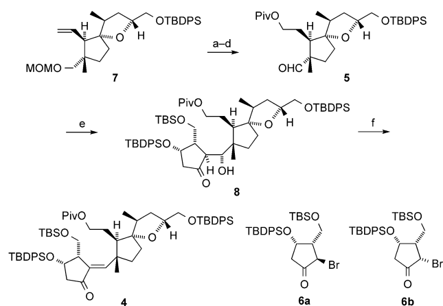
Scheme 2. Preparation of 4 . a) 9-BBN, THF, RT; then 3 M NaOH, 30% aqueous \text{H}_2\text{O}_2 , RT, 100%; b) PivCl, py, DMAP, \text{CH}_2\text{Cl}_2 , RT, 100%; c) \text{BF}_3 \cdot \text{OEt}_2 , \text{Me}_2\text{S} , \text{CH}_2\text{Cl}_2 , -30^\circ\text{C} , 92%; d) Dess–Martin periodinane, \text{CH}_2\text{Cl}_2 , RT, 94%; e) 6a or 6b (2.0 equiv), \text{Ph}_3\text{SnH} , \text{Et}_3\text{B} , benzene, RT, 90% (from 6a ), 83% (from 6b ); f) Burgess reagent, benzene, RT, 92%. 9-BBN = 9-borabicyclo[3.3.1]nonane, DMAP = 4-dimethylamino-pyridine, MOM = methoxymethyl, py = pyridine.
